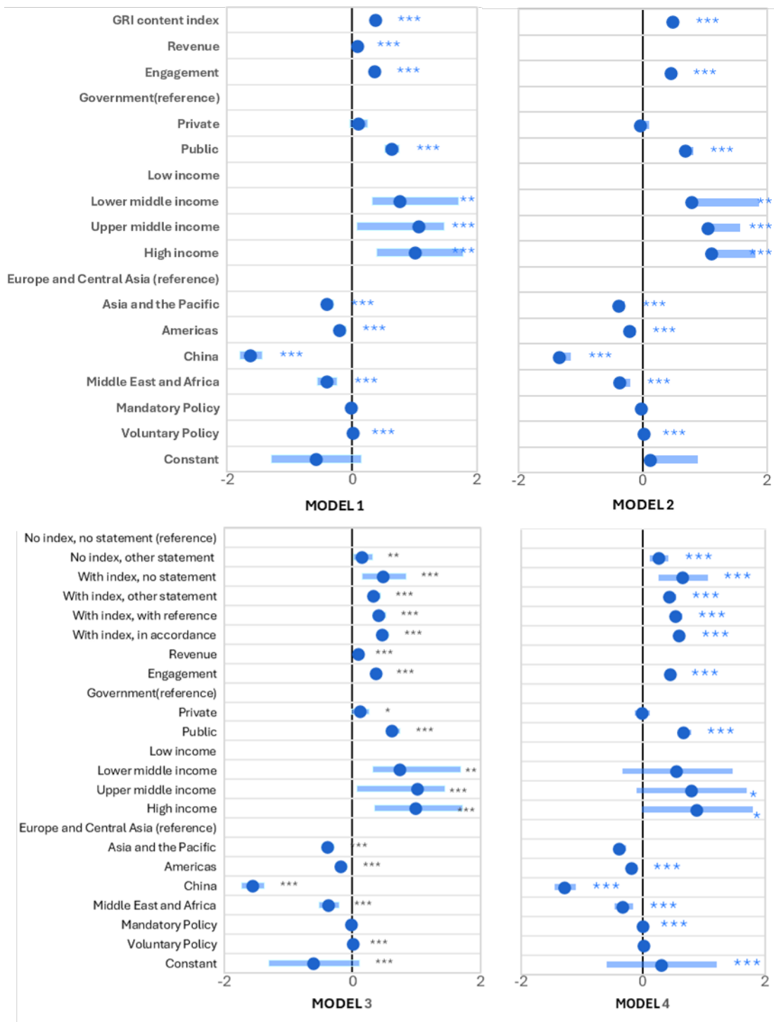
FIGURE 5: REGRESSION RESULTS
